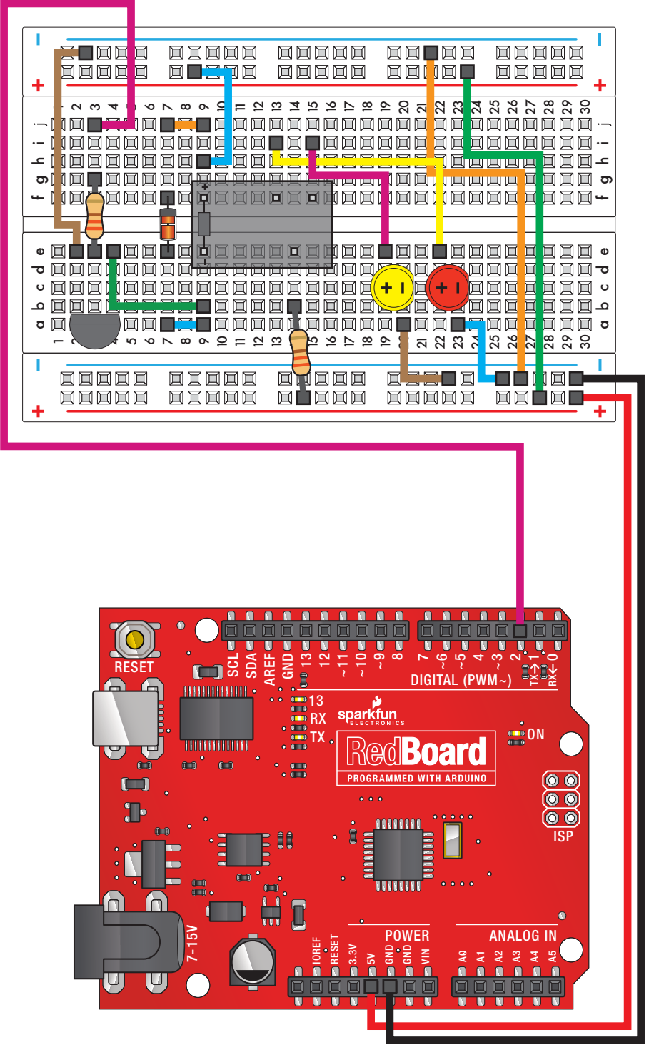
Circuit 13: Relays
